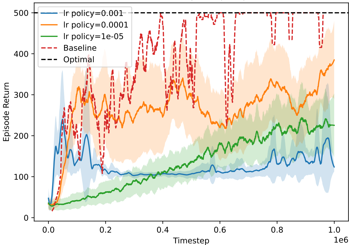
A2C learning rate policy
